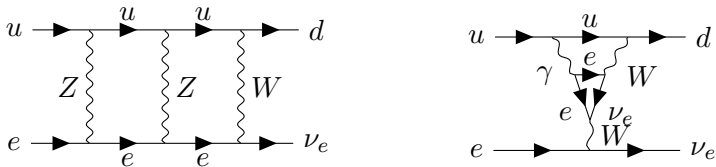
Figure 2: SM NNLO EW corrections.
