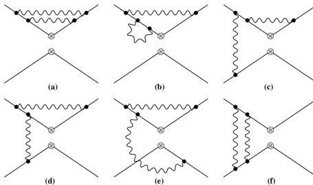
Figure 1: EFT NNLO EW corrections.
